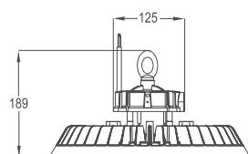
HELO PRO (L) 240W / 300W
