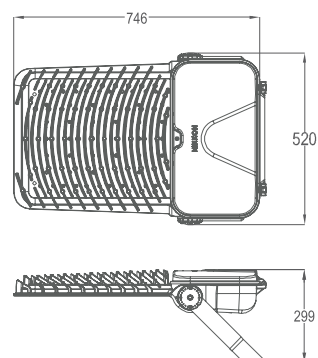
Mounting Bracket
