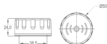
MOTION SENSOR
