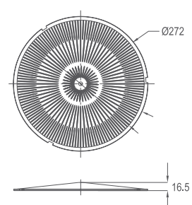
PC Visor
