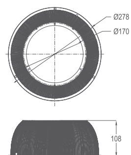
PC Reflector
