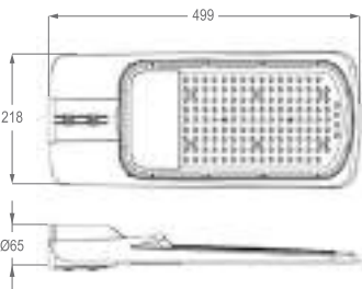
ALPHA 100W / 120W
