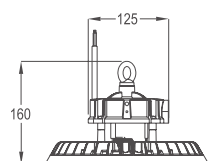
HELO PRO (XS) 100W
