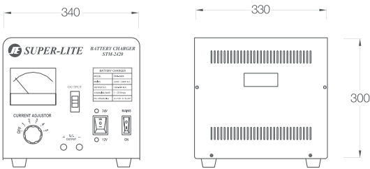
model: STM 2420
