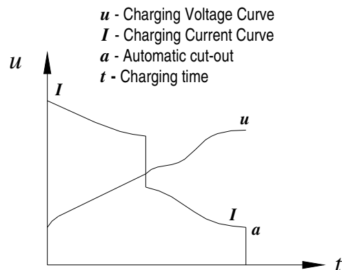
Charging curve against time
